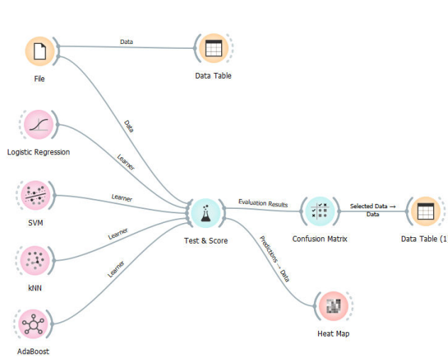
Figure 1. Work Flow Diagram for ML Algorithms
